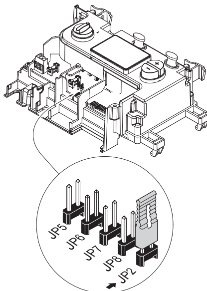
Fig. 8 Start-up delay
