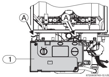
Fig. 1 Remove the control box
