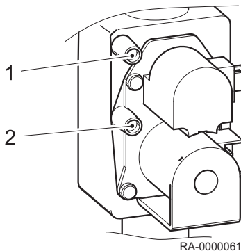
Abb.24 Gasventil WGB EVO
