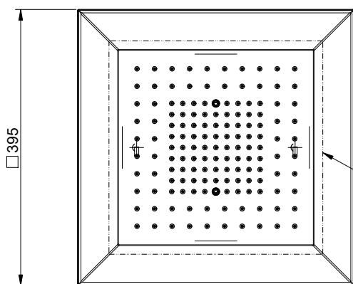
INSTALLATION MODE 1
