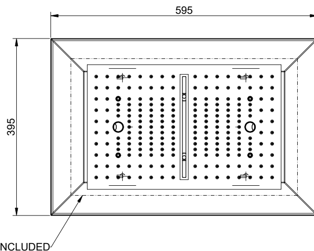
INSTALLATION MODE 2
