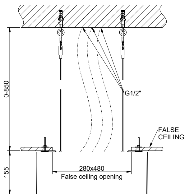
INSTALLATION MODE 1
